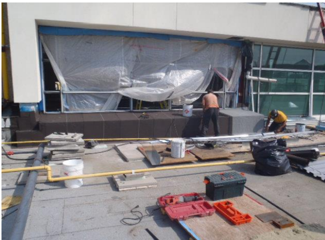
Detailing Work of Clerestory Flashings
